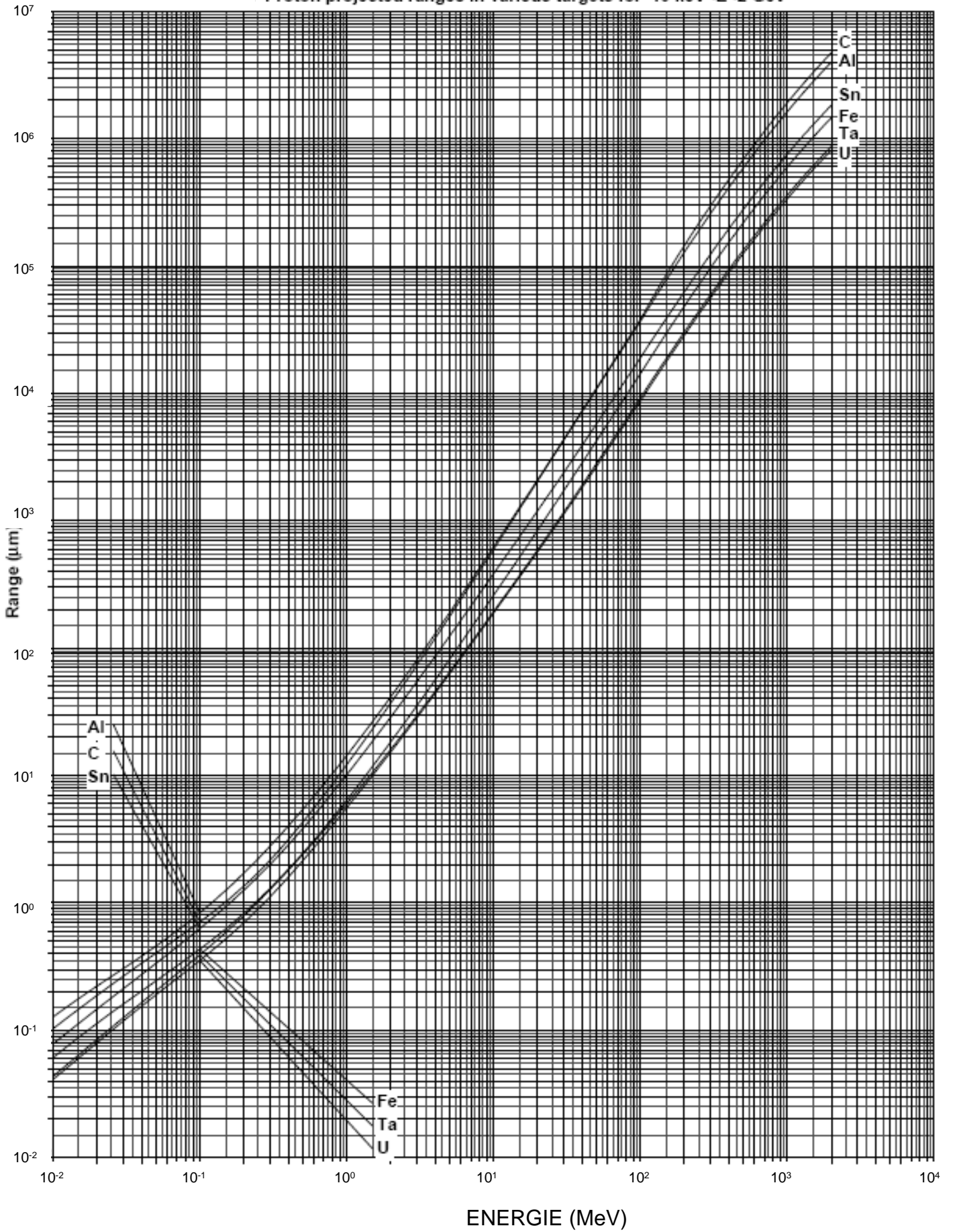
Proton projected ranges in various targets for 10 keV <math>E < 2 \text{ GeV}</math>
